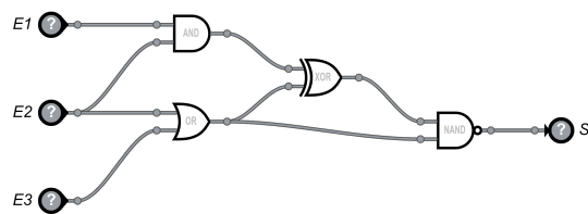
Figure 4: Circuit 1 maison
