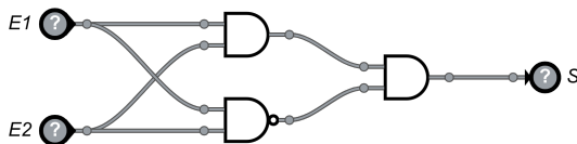
Figure 2: Circuit 2 cours
