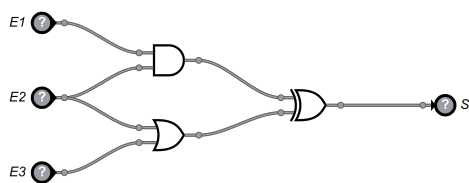
Figure 1: Circuit 1 cours
