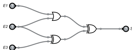
Figure 3: Circuit 3 cours
